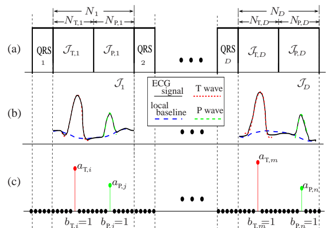
Fig. 1. ECG signal within a D -beat window: (a) QRS and non-QRS intervals (in this example, N_{T,n} = N_{P,n} = N_n/2 ), (b) signal in the non-QRS intervals, (c) impulse sequences u_{T,k} and u_{P,k} .
